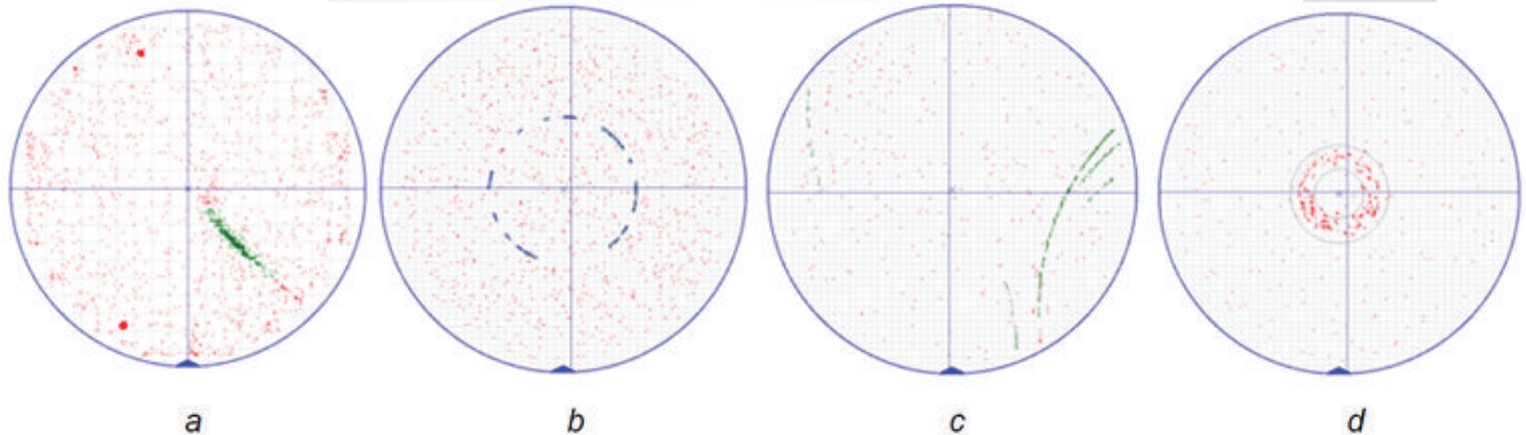
A defect spatial signature is a systematic distribution of defect on the surface of the wafer. The streak (a) and the circle (b) are identified using the object rules library. CMP scratches (c) are detected using a special scratch algorithm; a center ring is identified using zonal analysis.
